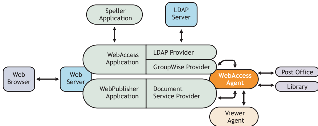
Figure 54-3 WebAccess Agent
