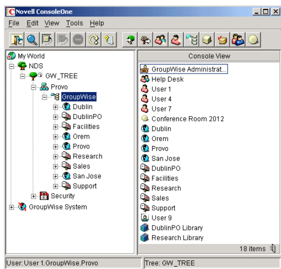
Figure 3-1 eDirectory View
