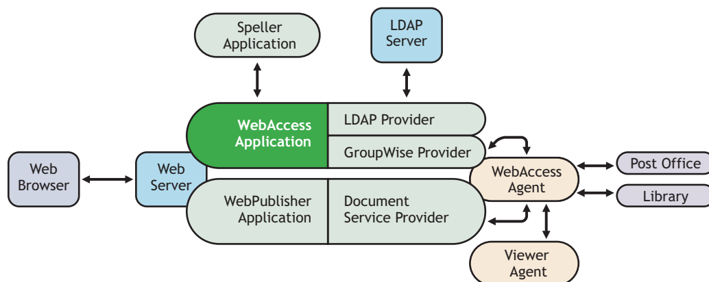
Figure 54-4 WebAccess Application
