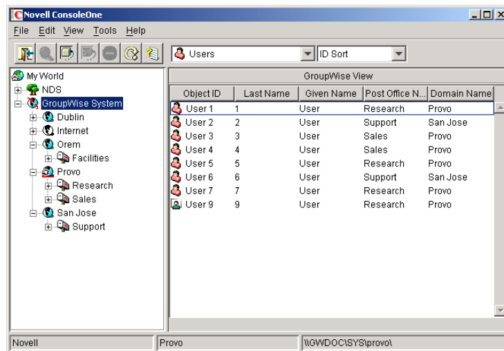
Figure 3-2 GroupWise View
