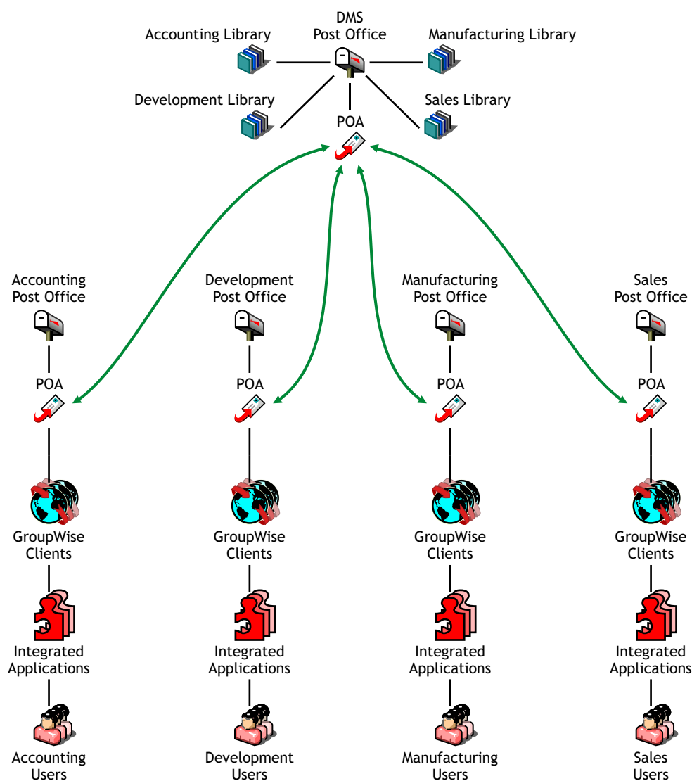
Figure 22-1 Centralized Libraries
