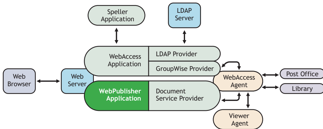
Figure 54-6 WebPublisher Application
