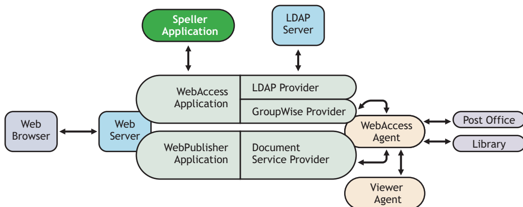
Figure 54-5 Speller Application
